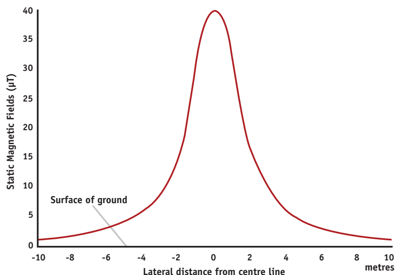
Figure D illustrates that the DC magnetic field decreases rapidly as you move away from the cable centre line. At a distance of 10 metres, the static magnetic field from the cable diminishes to 0.6μT. The DC magnetic field from this cable is far below the ICNIRP guideline (400,000μT).
